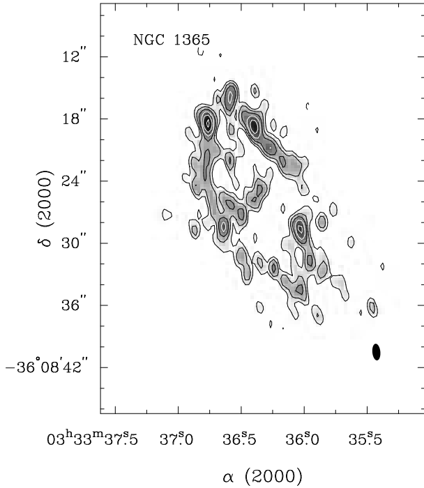
Fig. 6. NGC 1365. Contours: -0.6, -0.4, 0.4, 0.6, 0.9, 1.5, 2.3, 3.6 mJy beam -1
